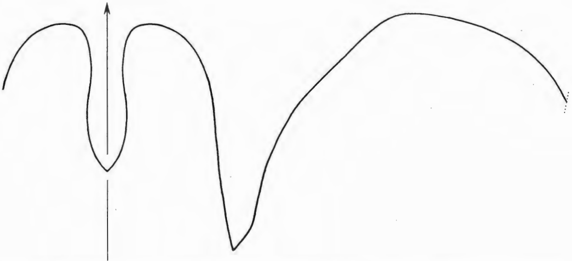
Abb. 35: Lobenlinie von Imitoceras ixion (HALL 1860); GPIT 1748/4748/1, Rockford Limestone, Rockford, Indiana; Dm 92 mm, Wb 31 mm, Wh 51 mm; x 2,5.
