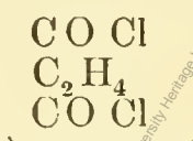
Succinylchlorür,
