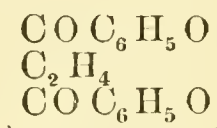
Succinylphenol,
