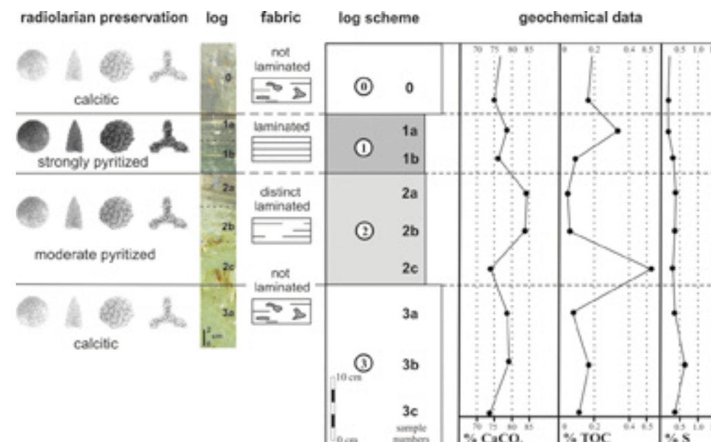
Fig. 4: The different preservational features of the radiolarian fauna. Correlated with the original log (longitudinal scan of the polished surface), the sediment fabric (laminated, distinct laminated and not laminated), and the geochemical parameters from the Sparbach section within and around the Karsteniceras Level.
