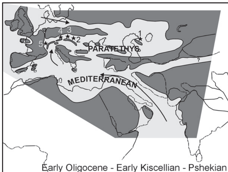
Fig. 1. Palaeogeographic map of the western Tethys (Mediterranean and Paratethys Seas) in the Early Oligocene (RÖGL 1998). Asterisks mark the sections with the occurrence of Thyromata curvisepa (SUBBOTINA, 1947): 1 – Northern Caucasus, 2 – North Hungarian Paleogene Basin, 3 – Waschberg Unit, Austria, 4 – Allochthonous Molasse and Lower Inn Valley, Austria, 5 – Prealps, France.
