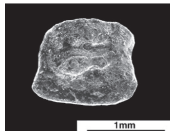
Fig. 3. Gobius brevis (AGASSIZ, 1839); right otolith, inner view, borehole Závod-72: 3,751-3,754 m, Karpatian, Vienna Basin.
