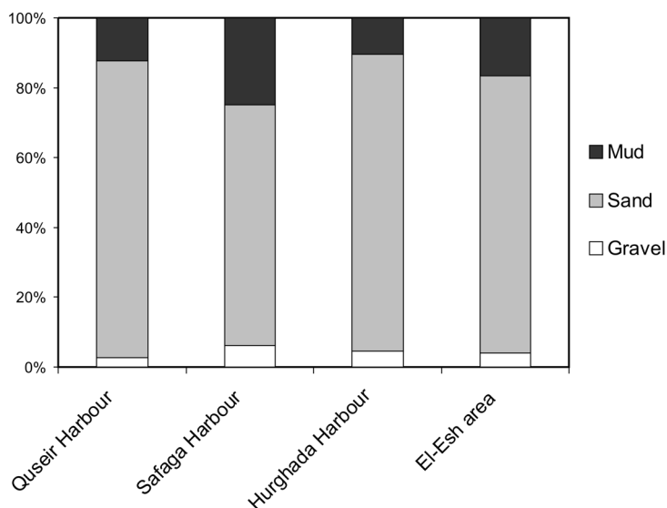
Fig. 4. Distribution of gravel, sand and mud fractions of coastal marine sediments of the studied localities.
