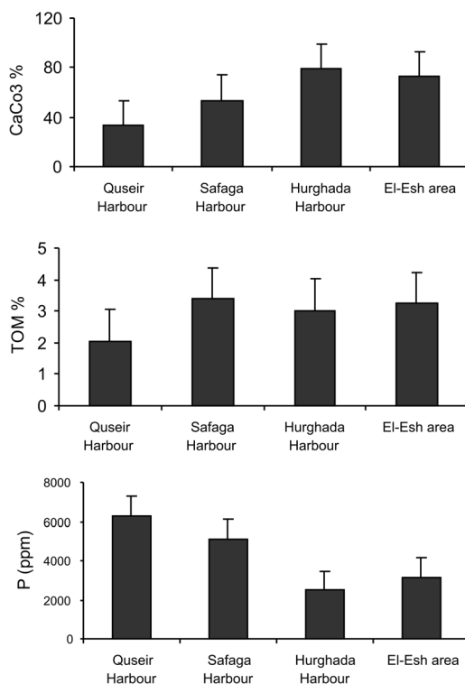
Fig. 5. Distribution of carbonate content, total organic matter, and phosphorus of coastal marine sediments of the studied localities.
