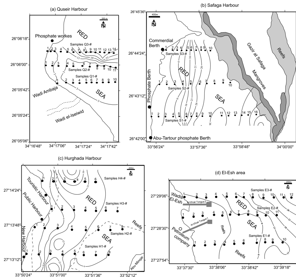
Fig. 2. Sample locations and bathymetric maps of (a) Harbours of Quseir, (b) Safaga, (c) Hurghada and (d) El-Esh area.
