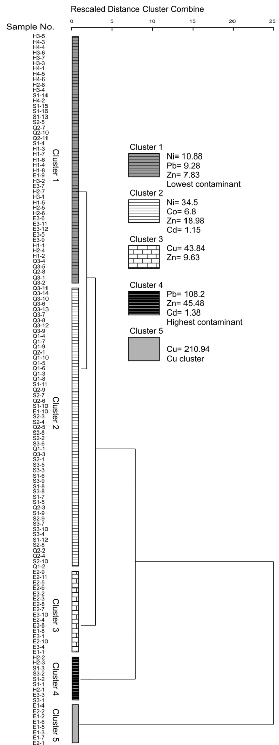
Fig. 7. Dendrogram from cluster analysis (Ward's method) of trace metals of sediment samples throughout the studied localities (compare Fig. 2).
