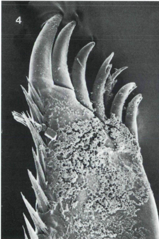
Abb. 4 - 5: Xeroporcellio pandazisi , ♀, Kefalliniá (SMNS T207). (4) Maxille I, Exit; (5) Maxille I, Endit.
