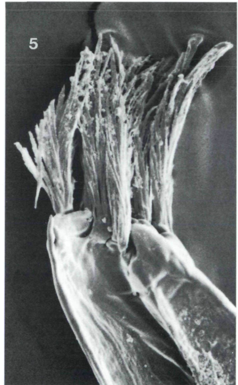
Abb. 4 - 5: Xeroporcellio pandazisi , ♀, Kefalliniá (SMNS T207). (4) Maxille I, Exit; (5) Maxille I, Endit.
