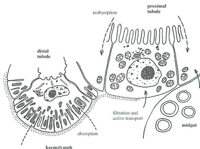
Fig. 27 Schema illustrating the transportation processes through the walls of the coxal gland tubules
