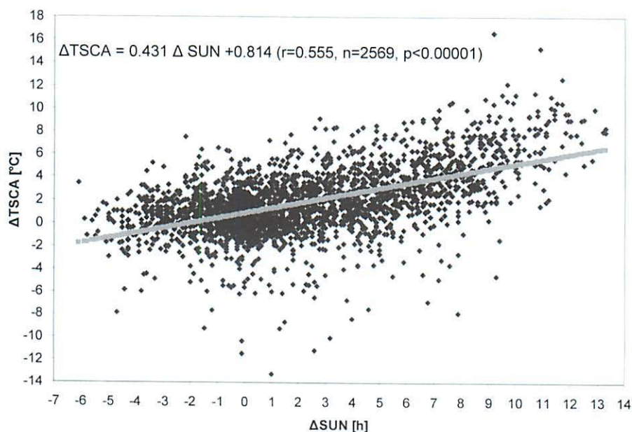
Fig. 4 Temperature change \Delta TSCA of air-temperature-corrected soil temperature above the seasonal mean plotted against the change of sunshine duration \Delta SUN of consecutive days from data sets of 54 German stations. Only data from radiation days with SUN \geq 9 of May to August 2003 were used.
