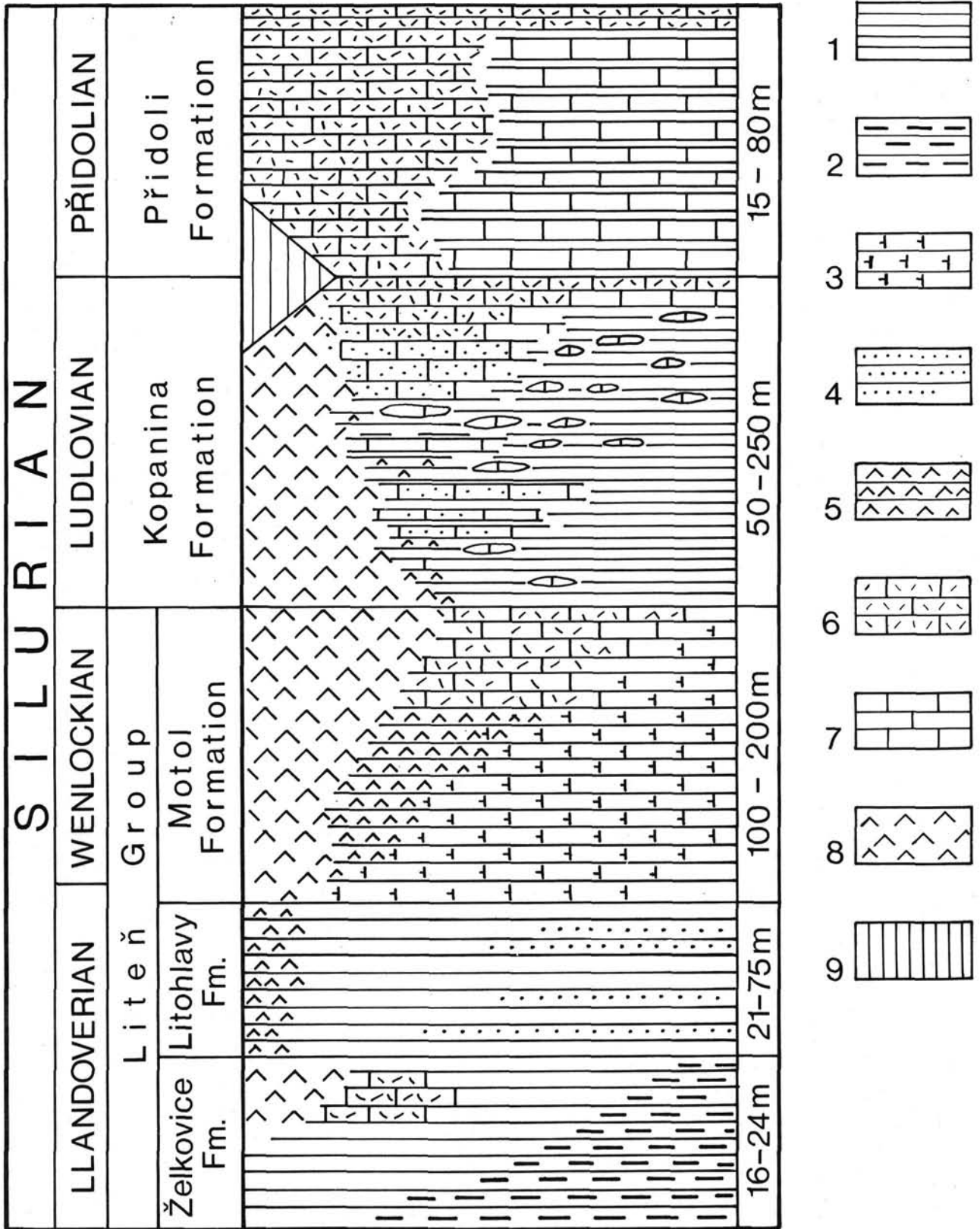
Fig. 2: Stratigraphic scheme of the Silurian in the Barrandian (according to R. HORNÝ 1962, J. KŘÍŽ, 1975): 1 – shales; 2 – shales with microcrystalline silicates; 3 – calcareous shales; 4 – alternating black shales and green claystones; 5 – tuffaceous shales; 6 – biosparites, biomicrites; 7 – micrites; 8 – volcanic rocks; 9 – stratigraphic break.
