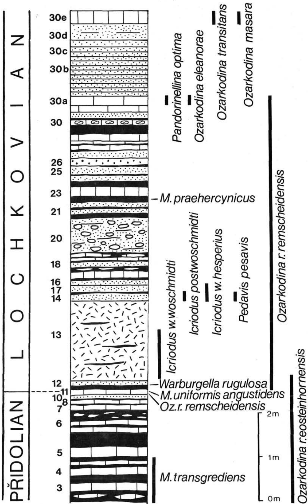
Fig. 7: Radotin Valley, „U topolu“, diagrammatic section of the Silurian-Devonian boundary interval (according to I. CHLUPÁČ et al. 1972, occurrence of conodonts after H. P. SCHÖNLAUB).
