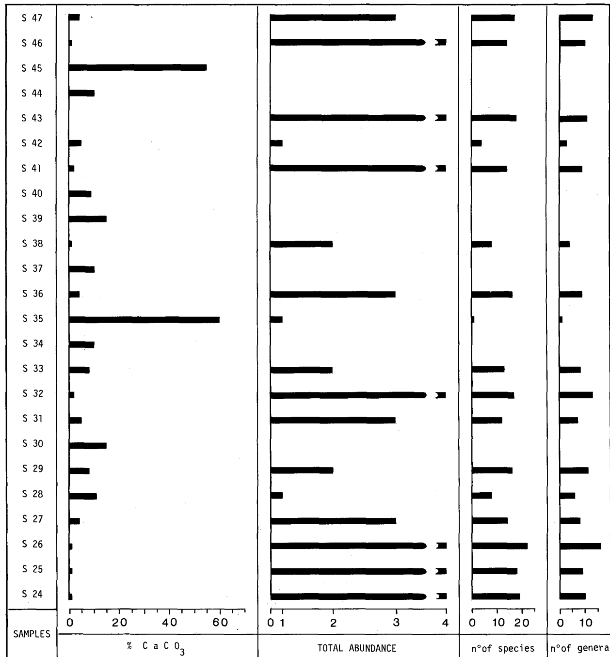
Fig. 5. Compared histograms of calcium carbonate percentage, total abundance, number of species and number of genera in Solignano Flysch samples.
