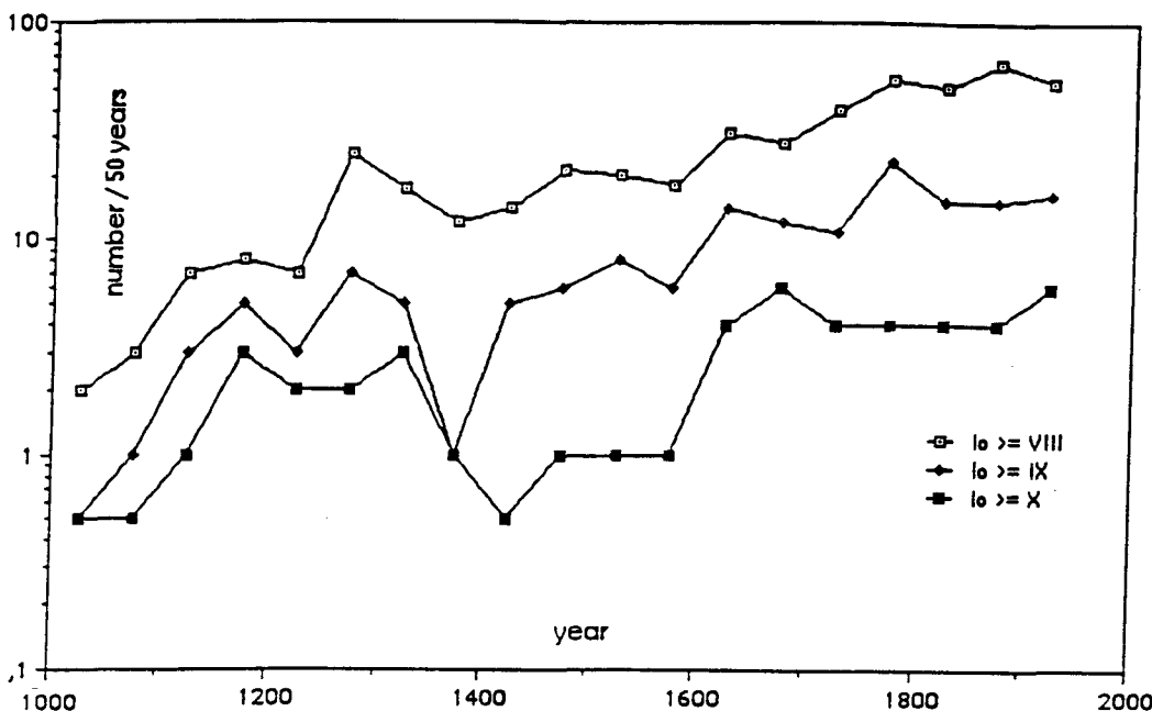
Figure 9. Number of earthquakes per 50 years in Italy. After POSTPISCHIL et. al. (1985).
