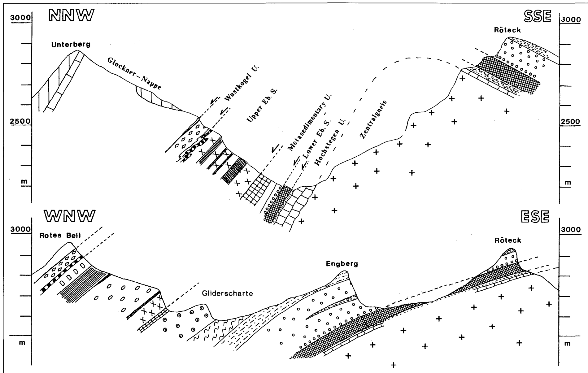
Fig. 3. Cross-sections (A,B) through the Unterberg-valley (horizontal equals vertical scale; symbols same as in Fig. 2). A: NNW-SSE section Unterberg-Rötack (central part of the valley); B: WNW-ESE section Rotes Beil-Rötack (southern crest).
