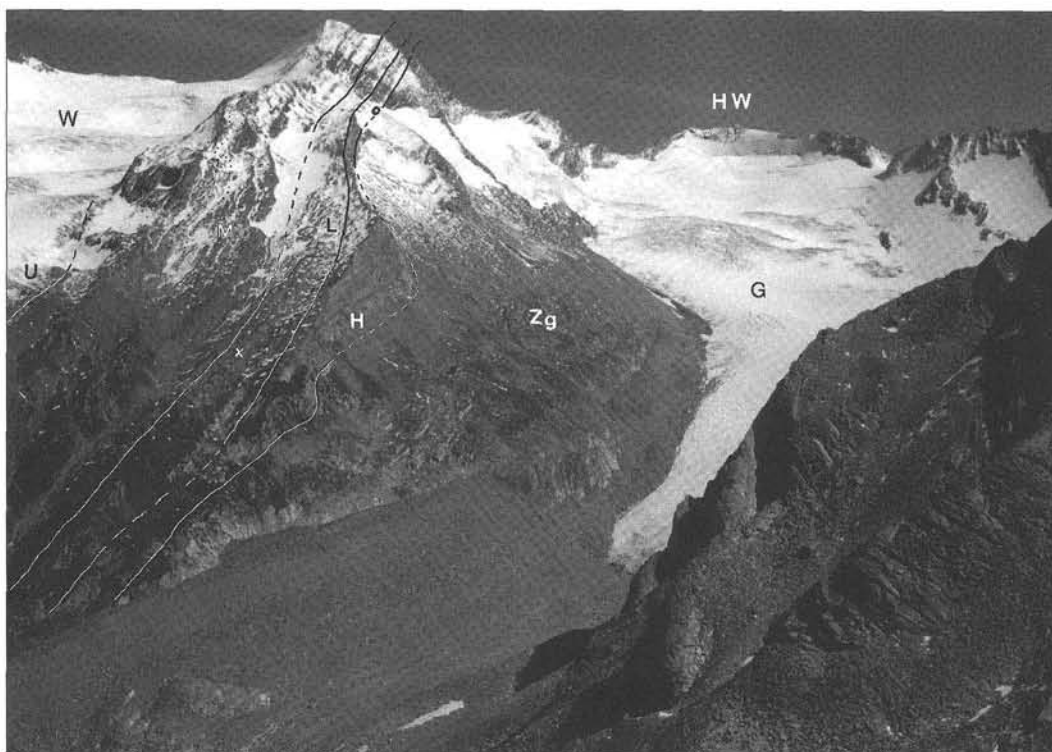
Fig. 4. View from Rôteck to the south-western ridge of Hochfeiler (left). HW = Hoher Weißzint, W = Weißkarferner, G = Gliderferner, Zg = Zentralgneis, H = Hochstegen-Unit, L = Lower Eisbrugg Slab, M = Metasedimentary Unit, U = Upper Eisbrugg Slab, Black circle = Liassic? Quartzite, x = Biotite Schist.
