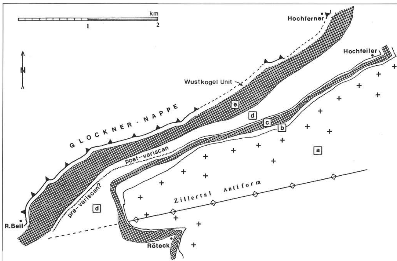
Fig. 15. Tectonic map of the working area showing main units of the Hochfeiler Duplex. a = Zillertal Zentralgneis Core, b = Hochstegen Unit, c = Lower Eisbrugg Slab, d = Paleozoic and Triassic Metasediments, e = Upper Eisbrugg Slab.
