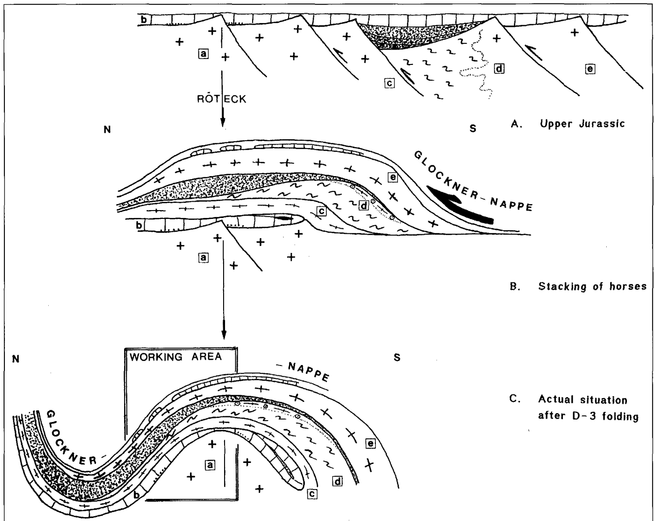
Fig. 17. Schematic sketch of the development of the Hochfeiler Duplex.
