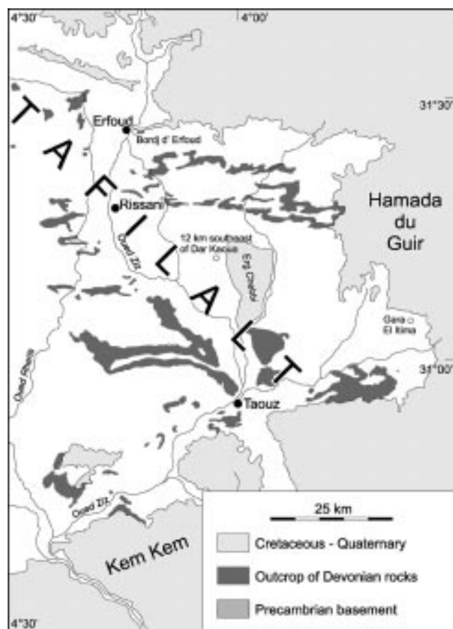
Text-Fig. 1. Location map of the goniatite-bearing localities in the Tafilalt (eastern Anti-Atlas, Morocco).
