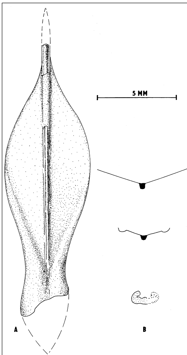
Text-Fig. 4. Gladius of Eoteuthoides n.g. – E. caudata . A: gladius. B: cross-section.
