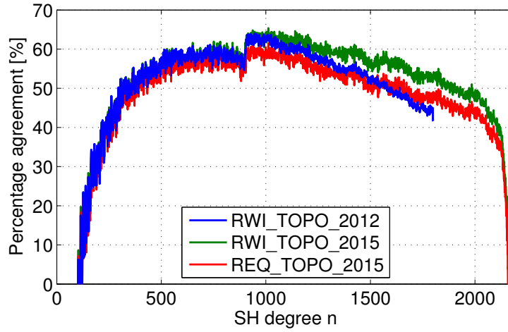
Fig. 16. Percentage agreement PA(n) of RWI_TOPO_2012 (blue curve), RWI_TOPO_2015 (green curve), and REQ_TOPO_2015 (red curve) with respect to EGM2008.
