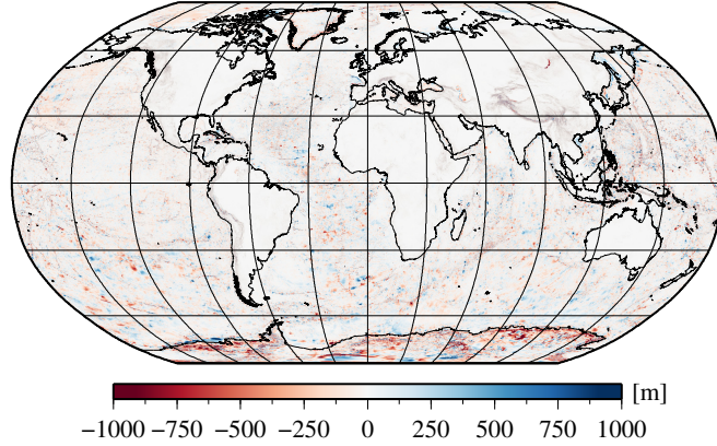
Fig. 4. Difference of the 1' \times 1' Earth2014 model and an interpolated version of the 5' \times 5' DTM2006.0 in terms of bedrock elevations. Robinson projection centered at 0^\circ longitude.
