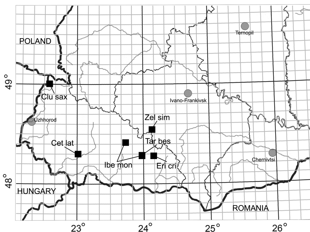
Fig. 2: Localities of species in the Ukrainian Carpathians: Clu sax – Clubiona saxatilis , Eri cri – Erigone cristatopalpus , Zel sim – Zelotes similis , Ibe mon – Iberina montana , Tar bes – Taranucnus bescidicus , Cet lat – Cetonana laticeps
