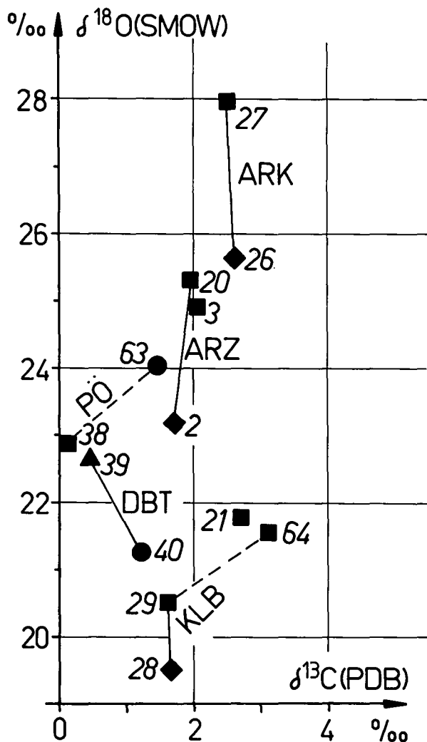
Fig. 6. The isotopic composition of cleft and host rock carbonates of five galena-sphalerite occurrences.
