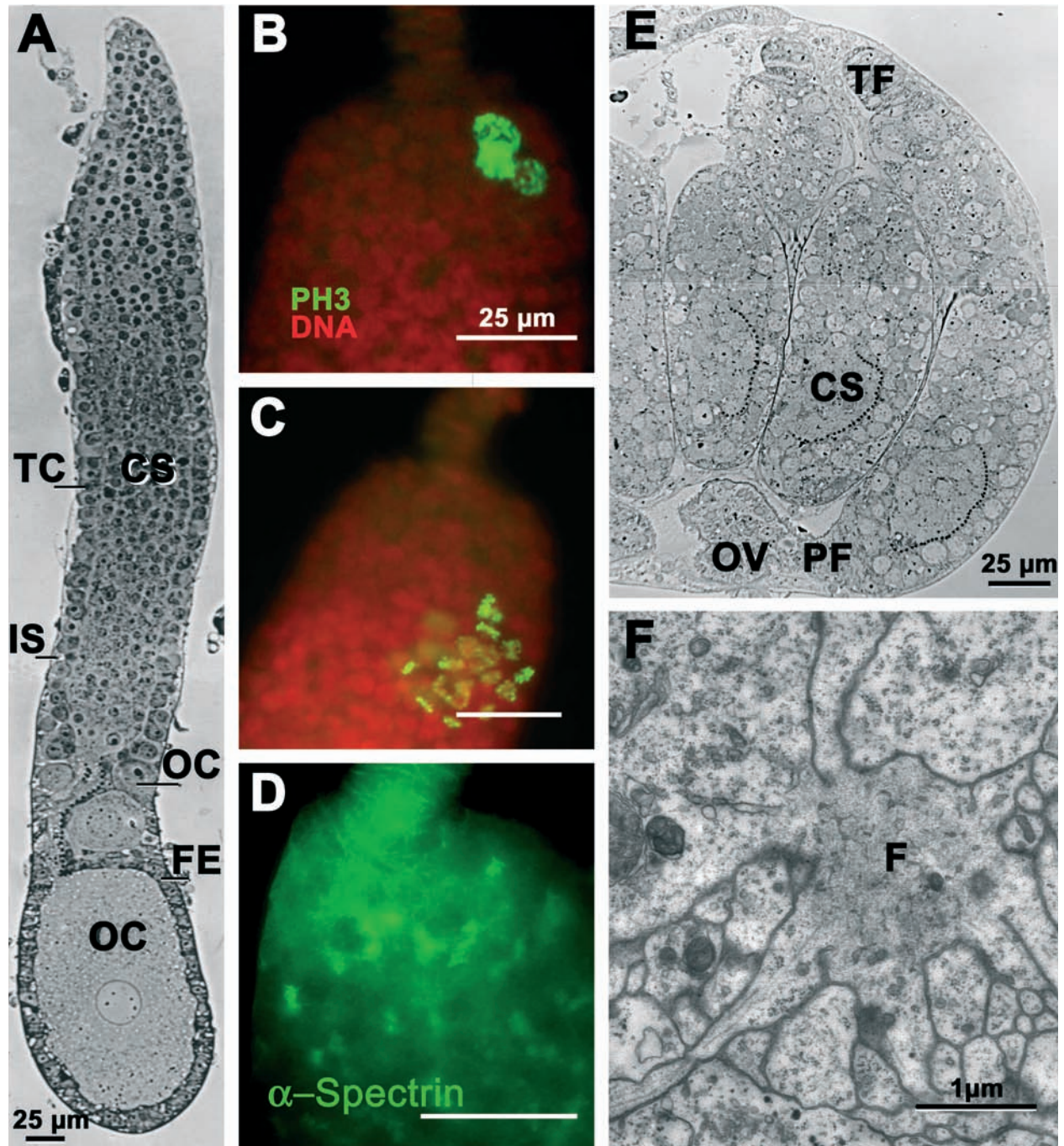
Fig. 5. Morphology and development of the Sialis -type telotrophic ovary. A: A functional ovariole of Raphidia flavipes (Raphidioptera) (BÜNING 1980). B–F: Larval ovarioles of Sialis sp. (Megaloptera). B,C: Fluorescence microscopy of anterior regions of larval ovarioles. Clusters arise in anterior regions; however, stem cell niches were not found. D: Clusters have polyfusomes as indicated by \alpha -spectrin labelling. E: Later in larval development, posterior clusters fuse and all inner membranes dissolve, giving birth to the central syncytium, bordered by single germ cells, the tapetum cells. F: The electron micrograph shows the centre of a cluster of cystocytes in which fusomal material accumulates (BÜNING 1979c, 1994; Rübsam & Büning in preparation). Abbreviations: TF (terminal filament), IS (inner sheath), TC (tapetum cell), CS (central syncytium), OC (oocyte), FE (follicular epithelium), PH3 (antibody against phosphohistone 3, a mitosis marker), F (fusome).
