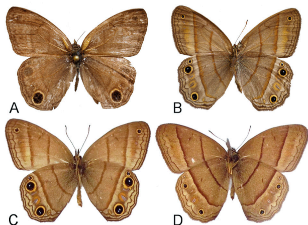
Fig. 6. Seasonal polyphenism in Cissia pompilia : A,B: Costa Rica, Puntarenas, Osa, collected in February: male: A – dorsal, B – ventral; C: Panama, collected in July (wet season): male; D: Mexico, collected in January (dry season): male. — © Trustees of the Natural History Museum, London.
