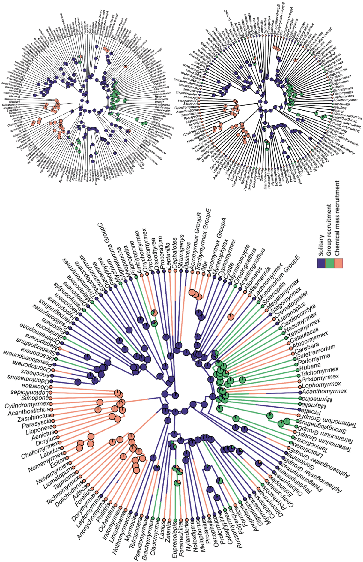
Fig. 4. Ancestral state reconstruction of LANAN (2014) foraging classifications. Clockwise from left: SCM; ML (polymorphic data); ML (monomorphic data).
