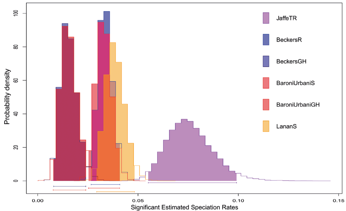
Fig. 5. Significant (non-zero) speciation rates from each analysis. TR = tandem running; R = recruitment; GH = group hunting; S = solitary. High speciation rates for group hunting may be due to the fact that the entirety of Dorylinae data were classified “group hunting” by Beckers et al. and Baroni Urbani classifications. The high speciation for tandem running is likely due to high transition rates for the behavior.
