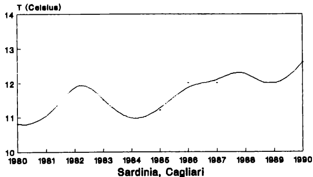
Fig. 2: Average minimum temperatures and interpolating curves of two southern Italian localities for 1980-1990 (data from Annuario Statistico Italiano, 1985, 1988, 1991, ISTAT, Rome).
