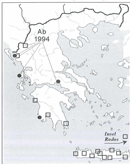
168. Spodoptera littoralis (BOISDUVAL)
