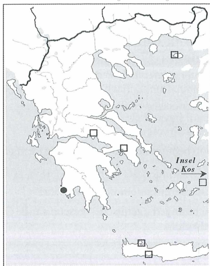
41. Tathorhynchus exsiccata (LED.)
