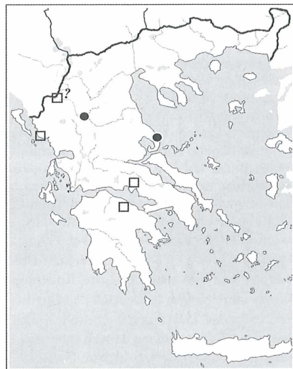
294. Noctua janthe (BORGHAUSEN)
