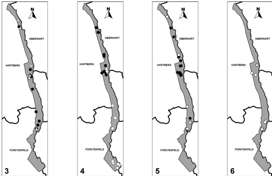
Abb. 3–6: Verbreitung im Lafnitztal. Distribution in the Lafnitz Valley . (3) \triangle Papilio machaon (Schwalbenschwanz / Swallowtail); \bullet Iphiclides podalirius (Segelfalter / Scarce Swallowtail). (4) \diamond Apatura ilia (Kleiner Schillerfalter / Lesser Purple Emperor); \circ Argynnis adippe (Feuriger Perlmutterfalter / High Brown Fritillary); \bullet Argynnis paphia (Kaisermantel / Silver-washed Fritillary). (5) \circ Boloria dia (Magerrasen-Perlmutterfalter / Weaver's Fritillary); \blacklozenge Boloria selene (Braunfleckiger-Perlmutterfalter / Small Pearl-bordered Fritillary). (6) \circ Brenthis daphne (Brombeer-Perlmutterfalter / Marbled Fritillary); \diamond Brenthis ino (Mädesüß-Perlmutterfalter / Lesser Marbled Fritillary).
