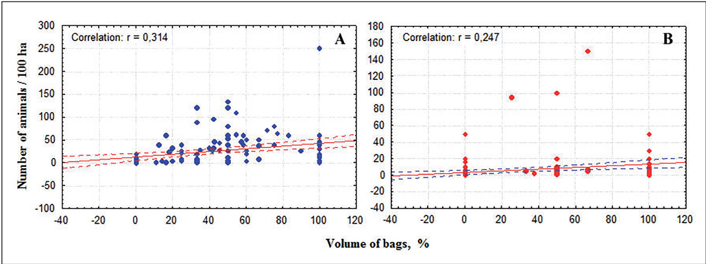
Fig. 7: The relationship between the hunting success and the population density of hares (A) and foxes (B)
