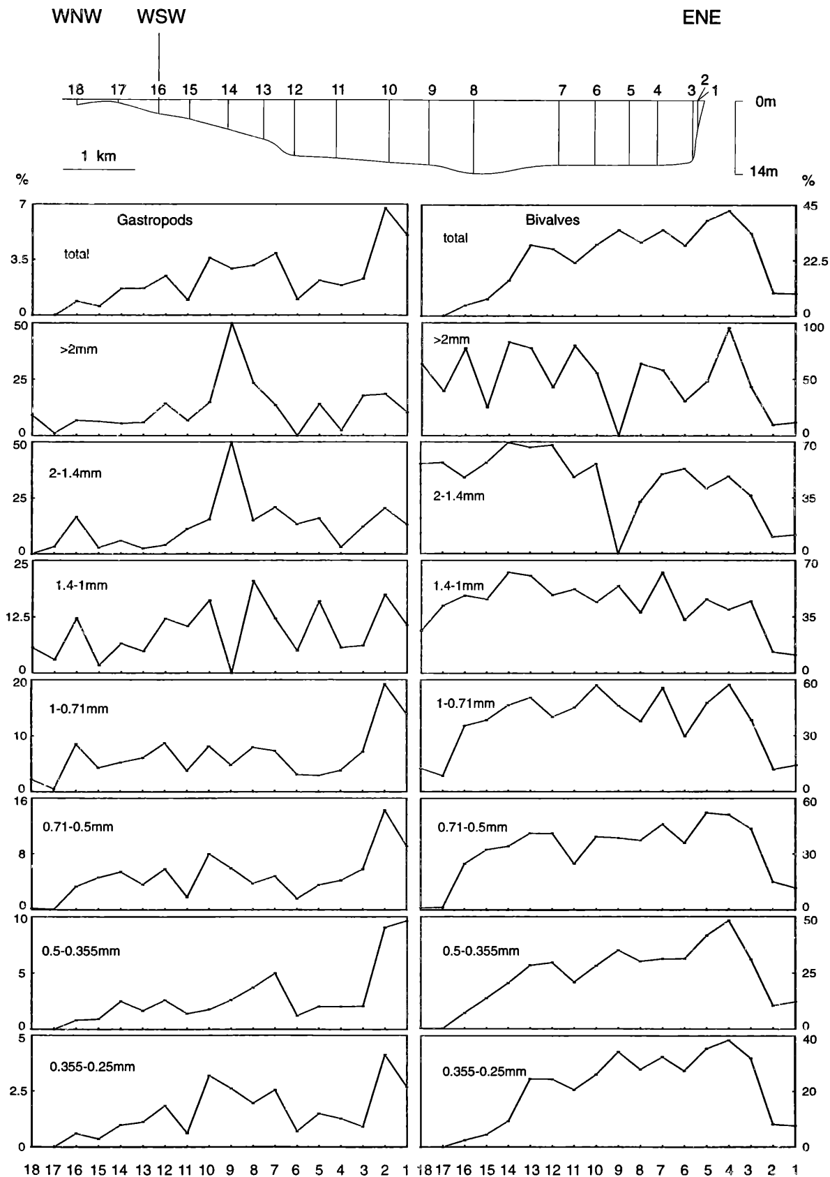
Fig. 14: Distribution of gastropods and bivalves in the sediment fraction > 250 \mu\text{m} and in each sieve fraction.
