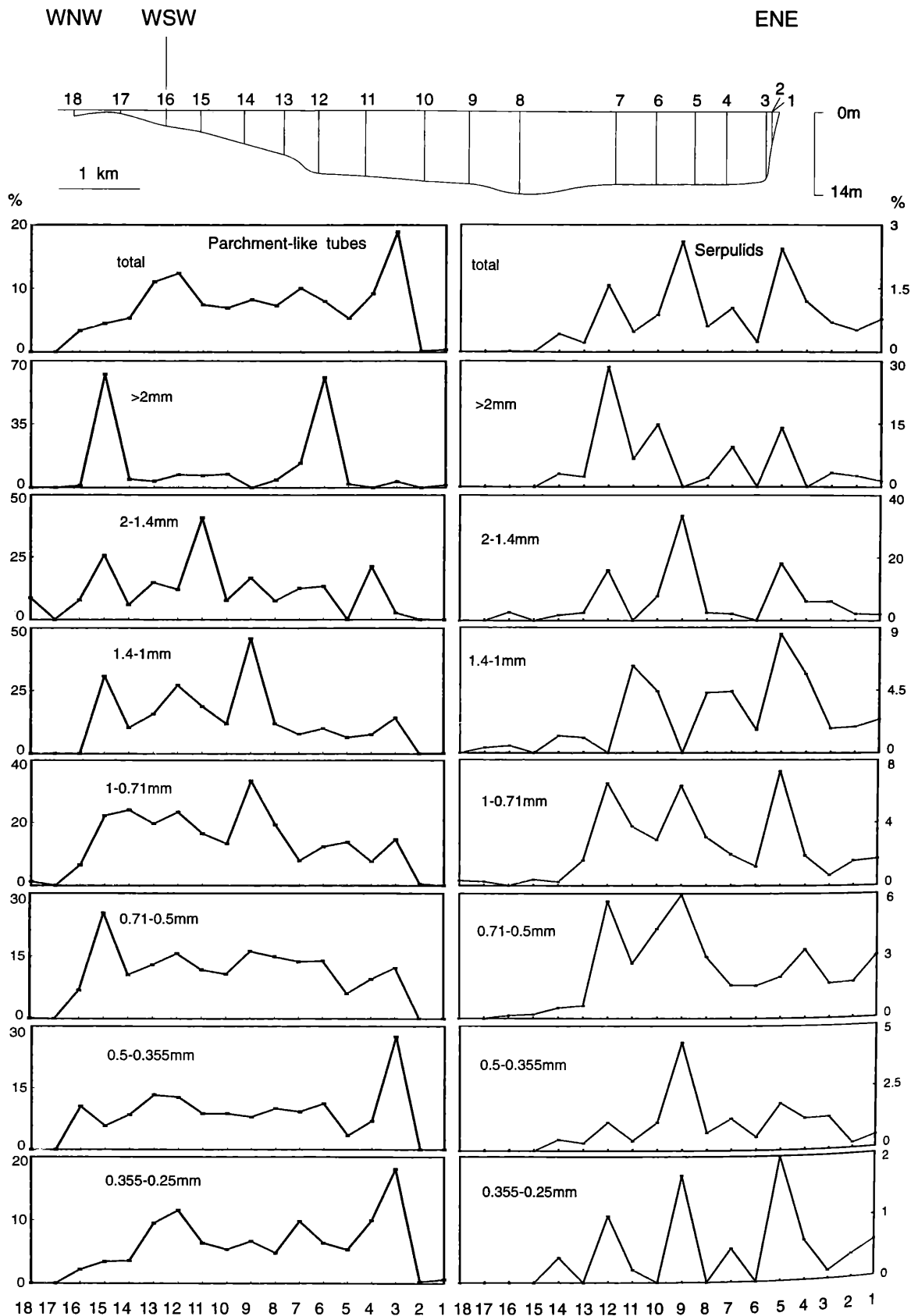
Fig. 16: Distribution of parchment-like tubes and serpulids in the sediment fraction > 250 \mu\text{m} and in each sieve fraction.
