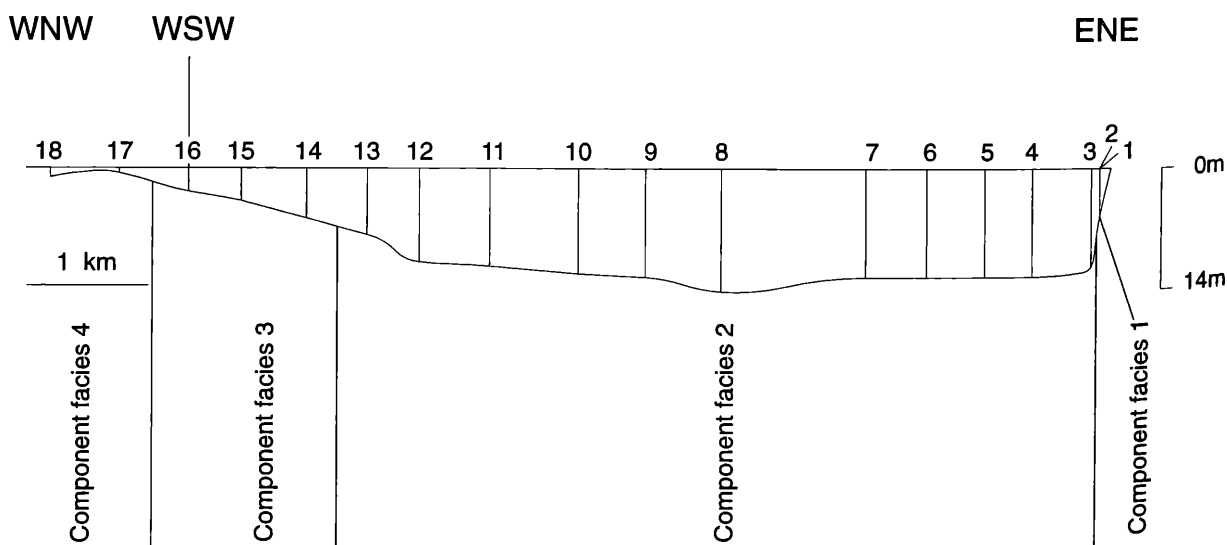
Fig. 18: Distribution of component facies along the transect.
