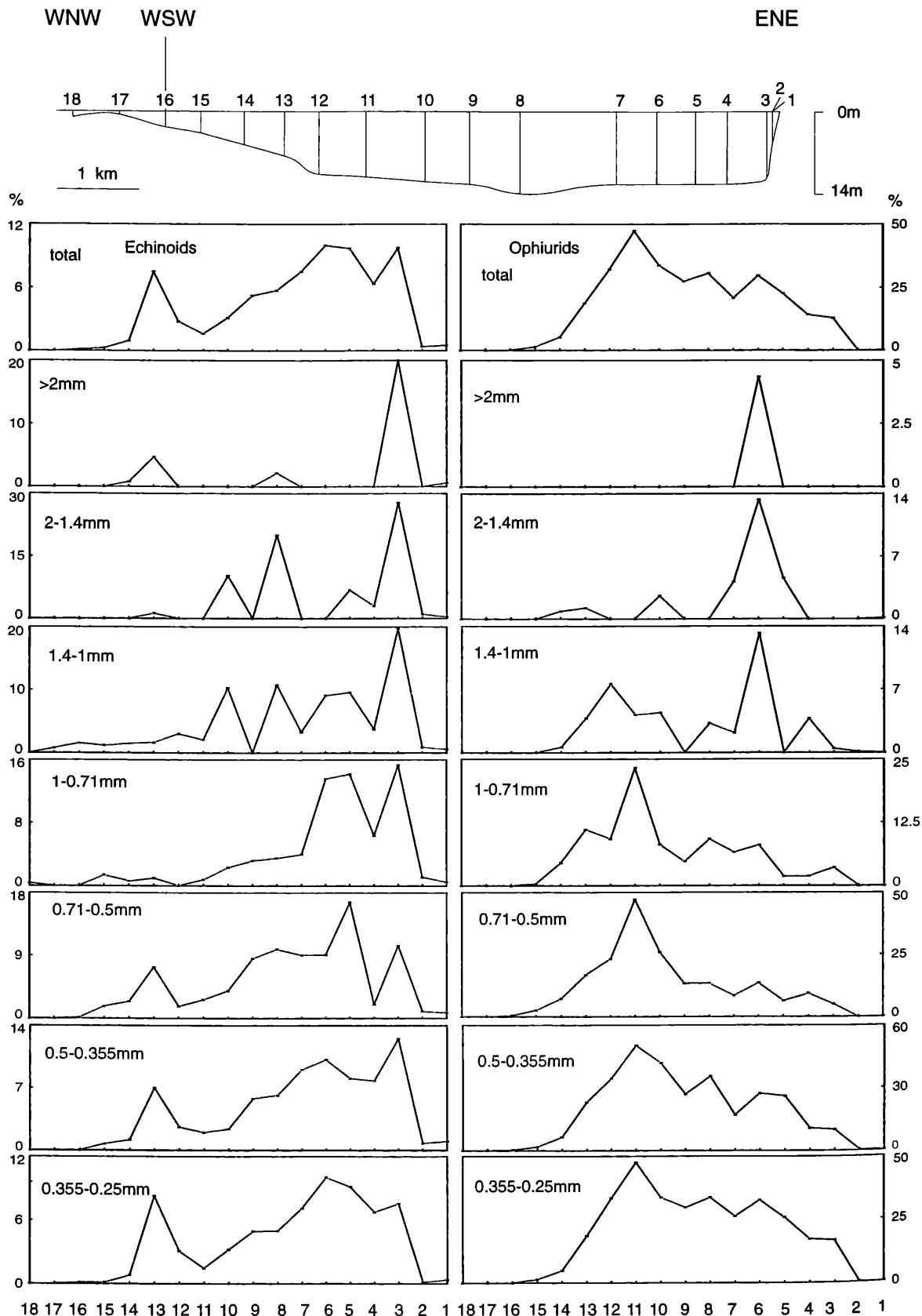
Fig. 15: Distribution of echinoids and ophiurids in the sediment fraction > 250 \mu\text{m} and in each sieve fraction.
