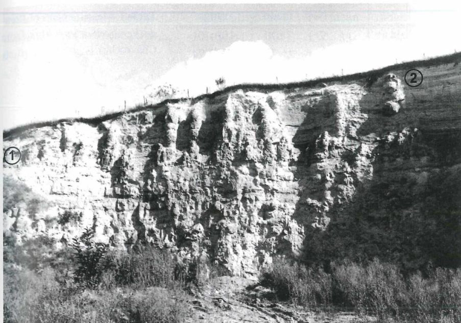
Figure 2: Cluzel quarry showing high Trichoptera columns embedded in marly layers. The first fossils came from the base of a column layer (= Cluzel 1); later, a higher level also yielded some teeth (= Cluzel 2).
