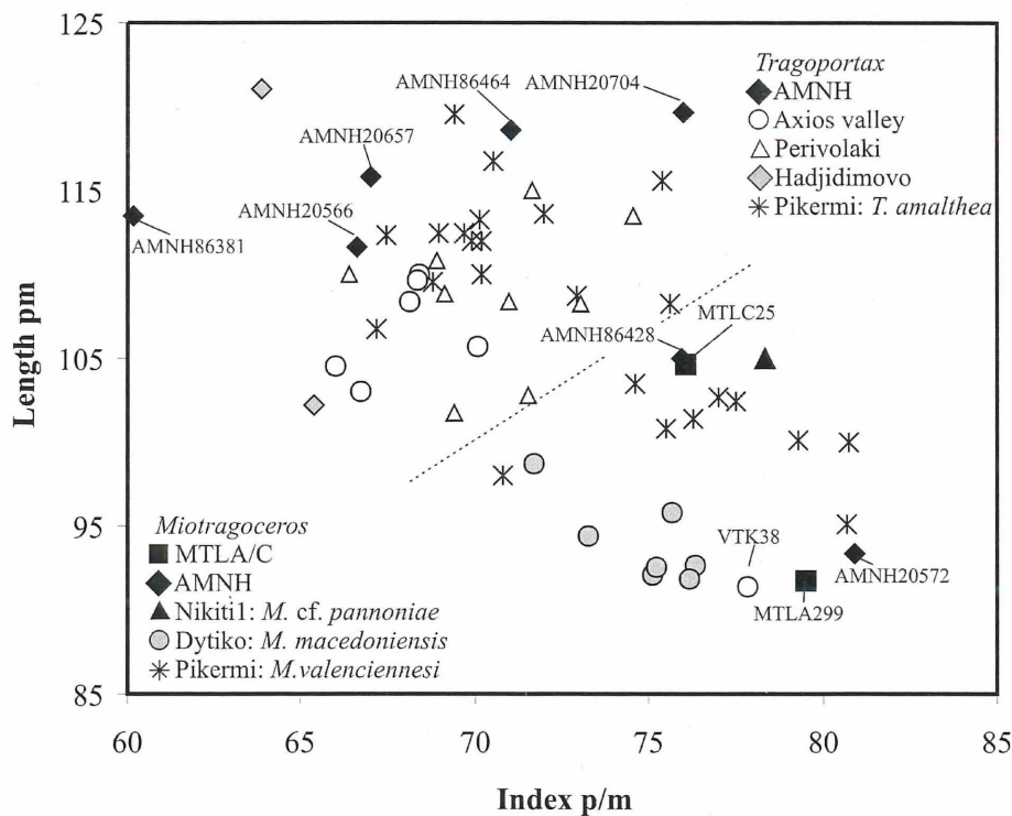
Figure 2: Scatter diagram comparing the lower premolar/molar ratio in relation to p2-m3 length of Miotragoceros and Tragoportax from several Balkan sites.
