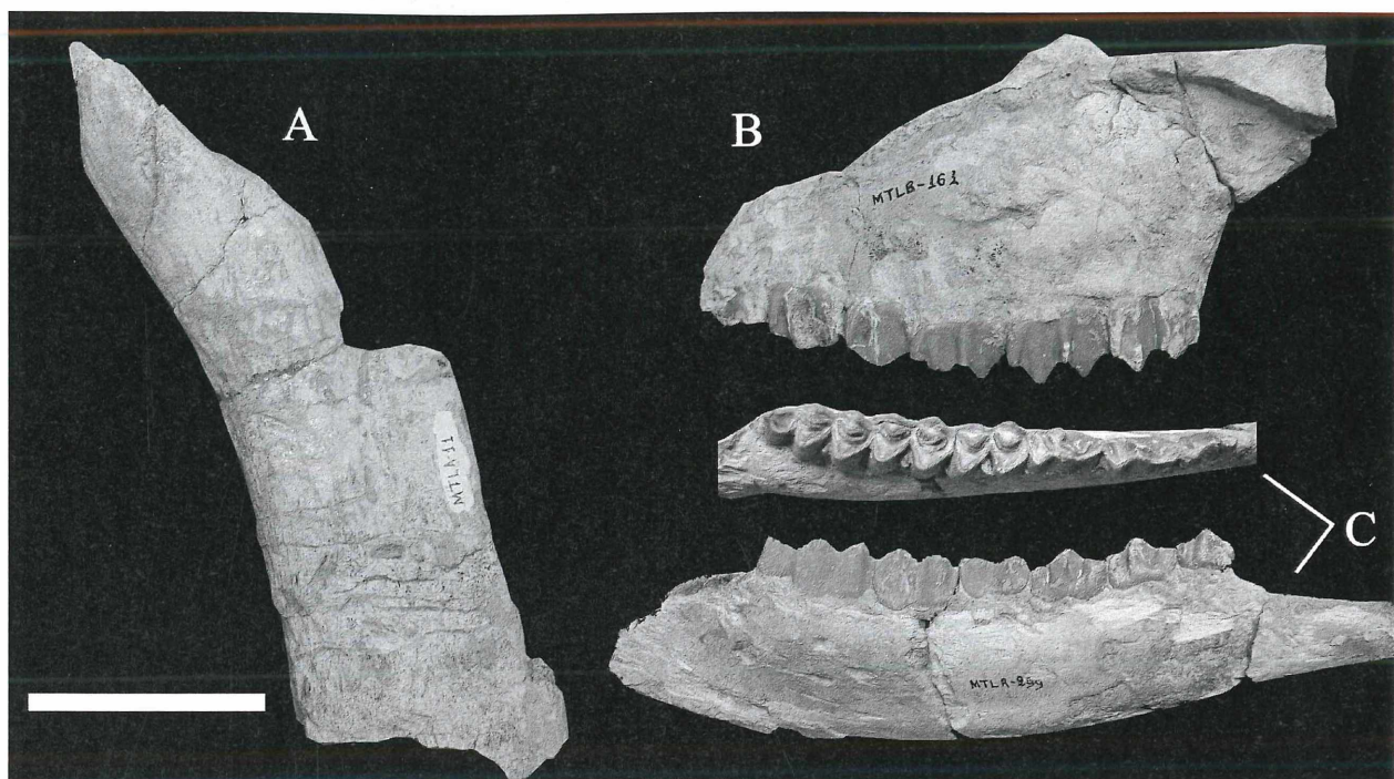
Figure 1: Miotragoceros valenciennesi from Samos. A. right horn-core, MTLA11 in lateral view; B. left maxilla, MTLB161 in buccal view; C. right mandible, MTLA299 in lingual and occlusal (reversed) view. Scale bar equals 5 cm.
