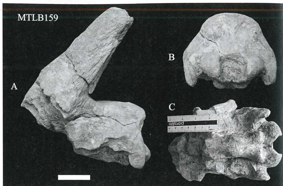
Figure 3: Tragoportax rugosifrons , cranium MTLB159 from Samos, in lateral (A), occipital (B) and basioccipital (C) view. Scale bar equals 5 cm.
