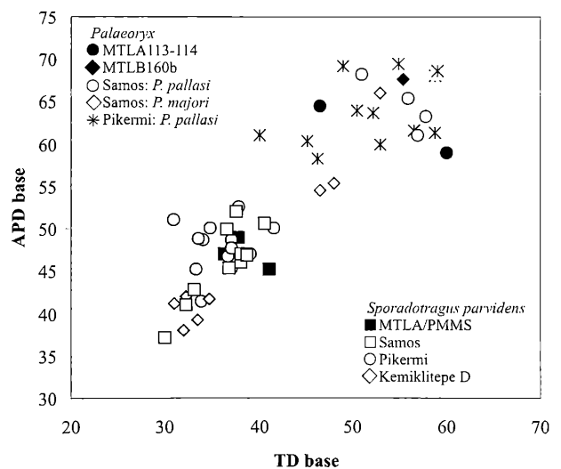
Figure 7: Scatter diagram comparing basal horn-core proportions of Sporadotragus parvidens and Palaeoryx from several sites.
