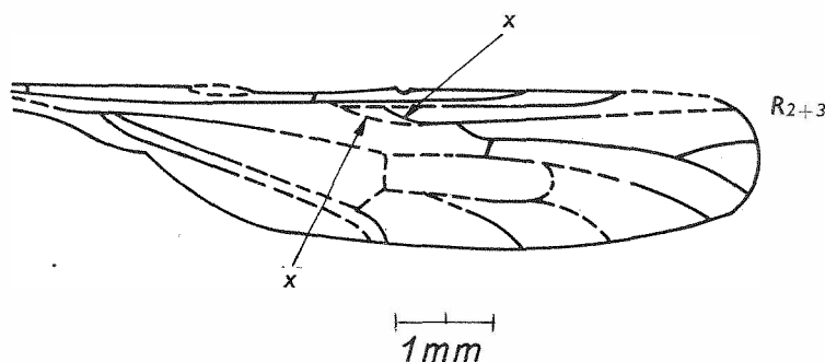
Fig. 2. The wing of Mesophantasma tipuliforme ROHDENDORF (After ROHDENDORF)
