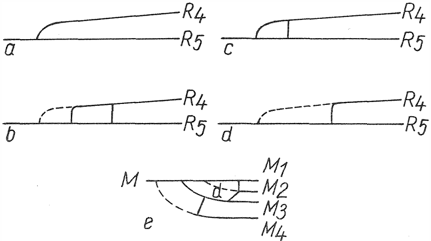
Fig. 1. The phases of the shift of longitudinal veins. Explanations in the text
