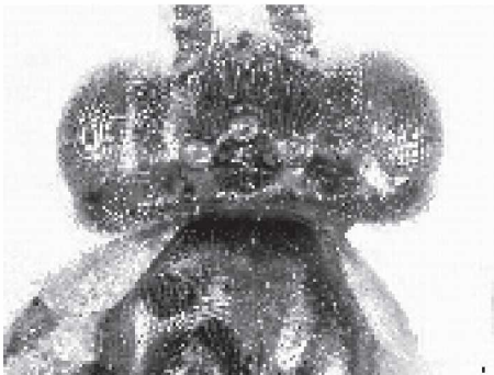
Fig. 9: Stauronematus saliciphilus sp. n. Female head and pronotum. Scale, 0.1 mm.
