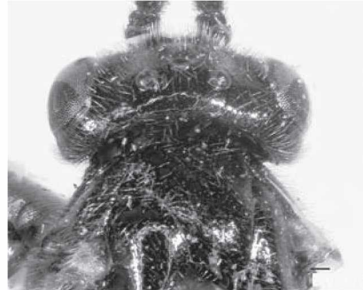
Fig. 7: Stauronematus platycerus (HARTIG). Male head and pronotum. Scale, 0.1 mm.
