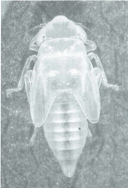
Figs 1-2: 5 th instar nymph of Zyginella pulchra Löw, 1885.
