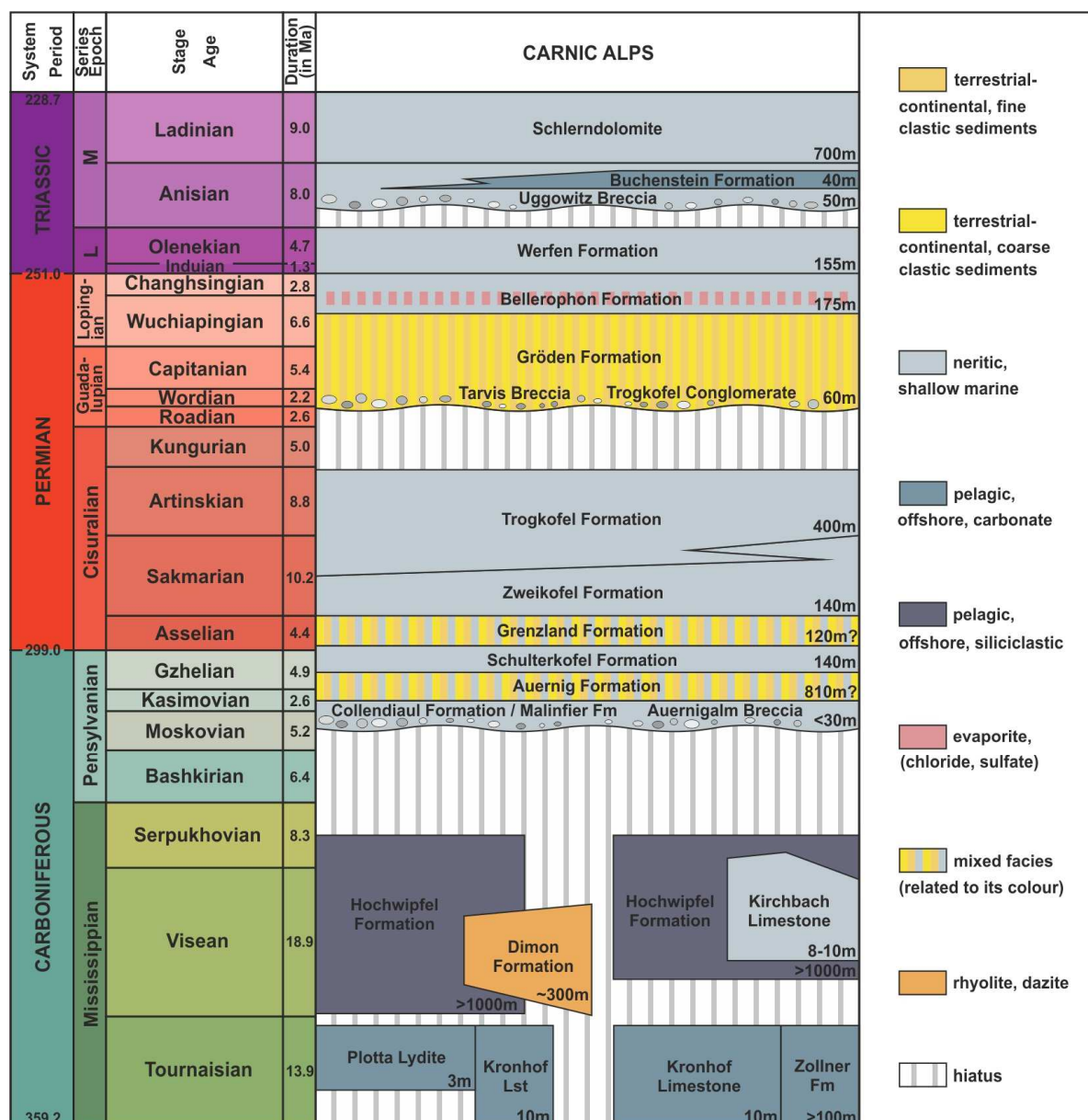
Fig. 2: Stratigraphic chart of Early Carboniferous (pre-Variscan sequence; after PILLER et al., 2004) and Late Carboniferous–Middle Triassic (post-Variscan sequence; after SCHÖNLAUB & FORKE, 2007) units in the Carnic Alps. The hiatus between the Serpukhovian–Moskovian stages demarcates the Variscan orogeny.
