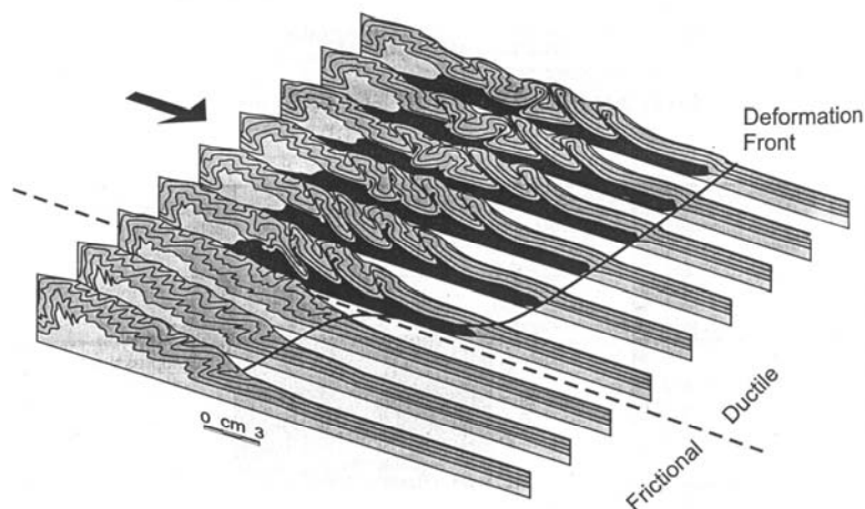
Analogue model showing the lateral termination of an low viscosity detachment layer. (Cotton and Koyi, 2000)
