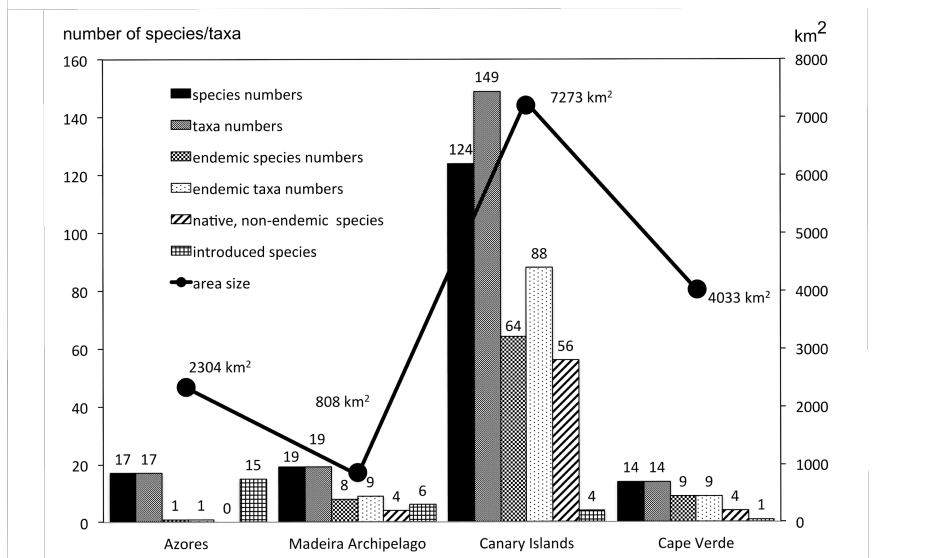
Fig. 4: Number of wild-bee species/taxa of the Archipelagos of Macaronesia (y-axis 1; total species/taxa numbers, endemic, native non-endemic, introduced species/taxa are differentiated. Area sizes (km²) of the specific archipelagos are indicated (y-axis 2).
