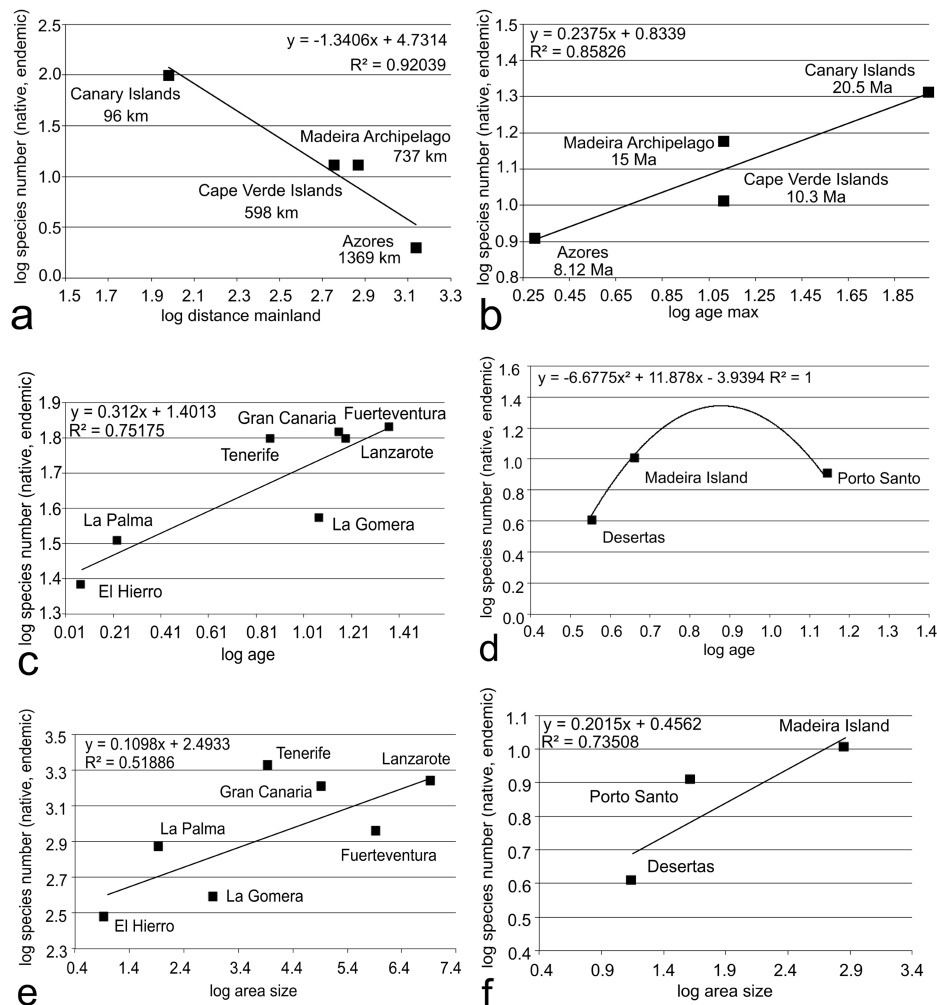
Fig. 5: Correlation (log-log) between the number of native and endemic wild-bee species and a) distance of a colonisation source of the different archipelagos; b) maximum age of the different archipelagos; c) age of the different islands of the Canary Islands; d) age of the different islands of the Madeira Archipelago; e) area size of the different islands of the Canary Islands; and f) area size of the different islands of the Madeira Archipelago.
