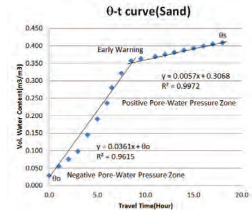
Figure: soil chamber test (top), \theta -t curve measured by soil chamber test (bottom).
