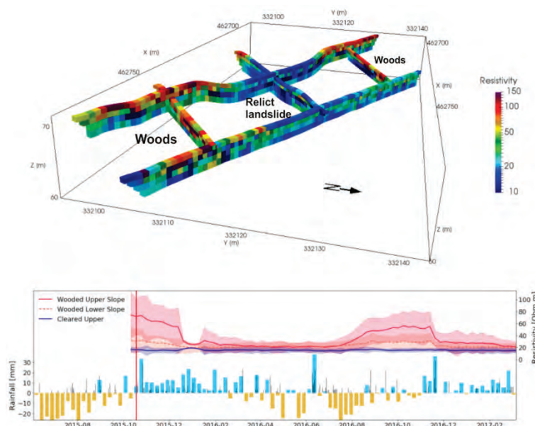
Figure 1: Resistivity baseline image, showing low resistivities of the relict landslide and high resistivities in the wooded areas. Lower panel shows resistivity dynamics and effective rainfall.
