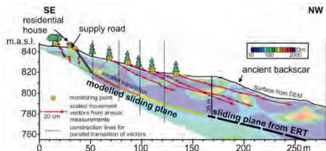
Figure: Cross-section of the northern Fürstberg ridge with ERT inversion results. For the sliding plane construction each movement vector is translated parallel into depth, starting with a sliding plane geometry interpreted from ERT inversion results.
