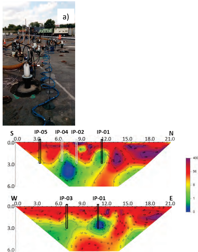
Figure: (a) Photo of ERT line (blue cable) installed on site. (b) S-N and W-E cross sections of ERT background independent inversion.
