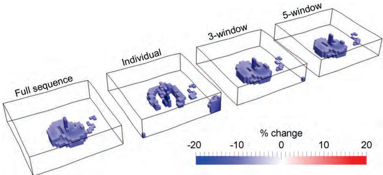
Figure 1: Resistivity changes caused by a controlled water leak in a monitoring experiment (cut-off at -10%). 4D temporally regularized inversions using moving windows of length 3 and 5 show much greater similarity to the full sequence inversion than individual standalone inversions without temporal constraints.
