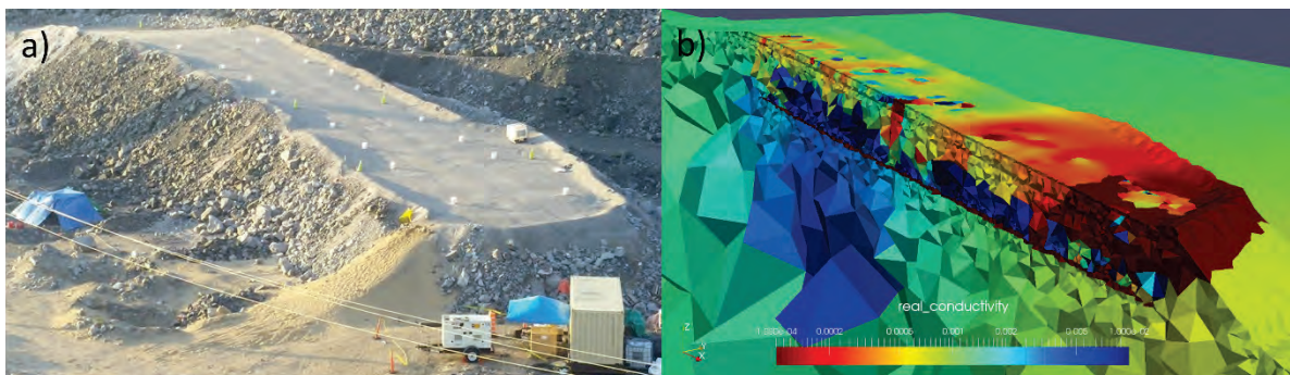
Figure: a) Photography of the experimental waste rock pile instrumented with 192 geophysical electrodes; b) 3D resistivity model of the pile: red areas correspond to the resistive sand and anorthosite while blue areas correspond to conductive ilmenite-rich waste rock.
