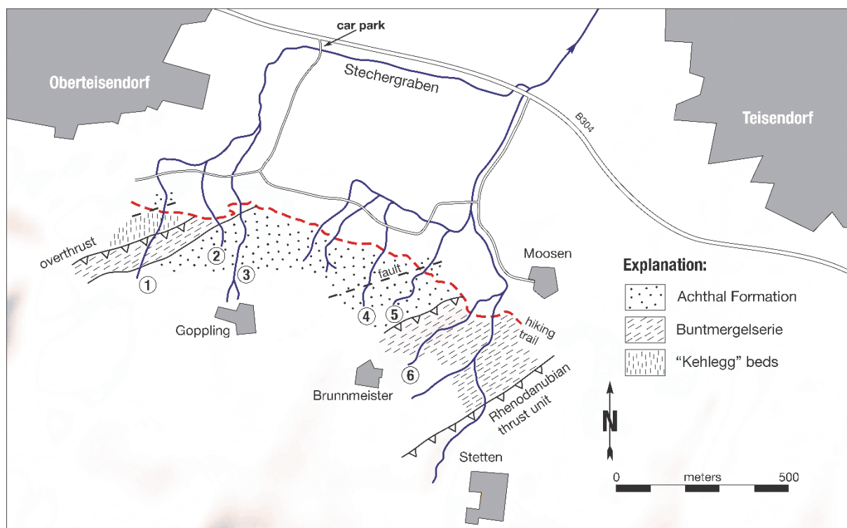
Fig. 23: Sketch map of the area investigated. Numbers indicate the most important creek sections mentioned in the text.
