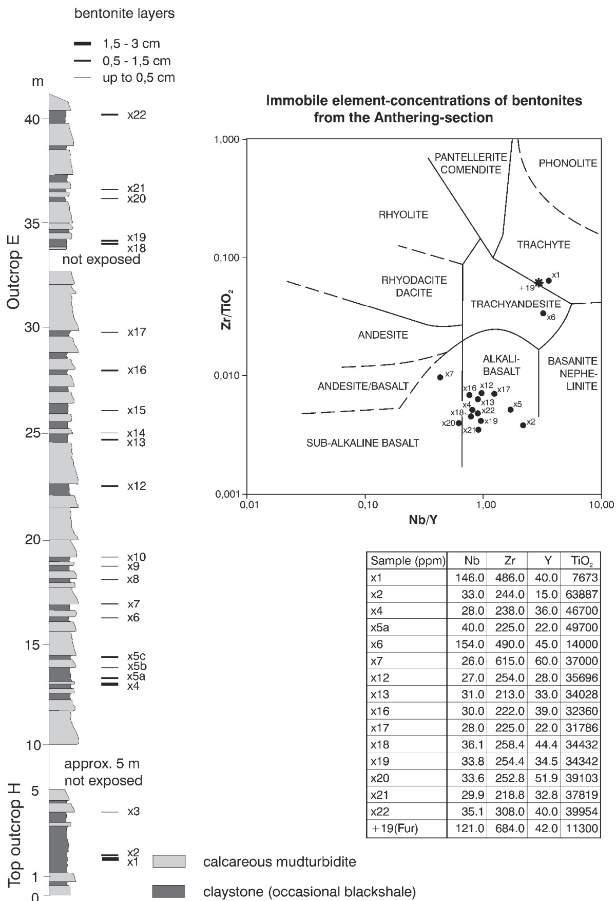
Fig. 15: Log of outcrop E showing positions of bentonites and immobile element concentrations of bentonites.
