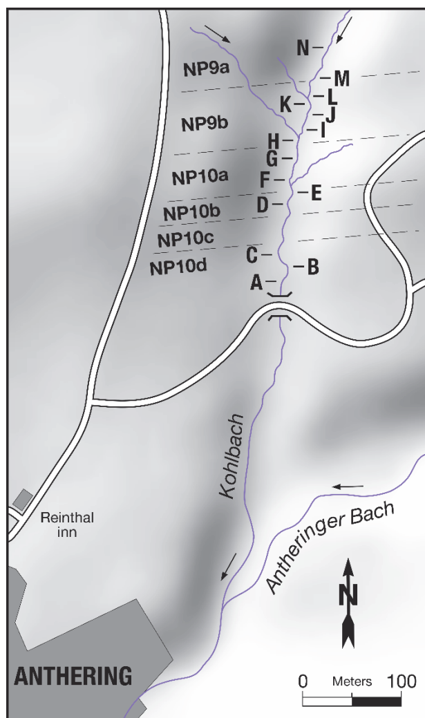
Fig. 11: Location of outcrops and biostratigraphy of the Anthering section.
