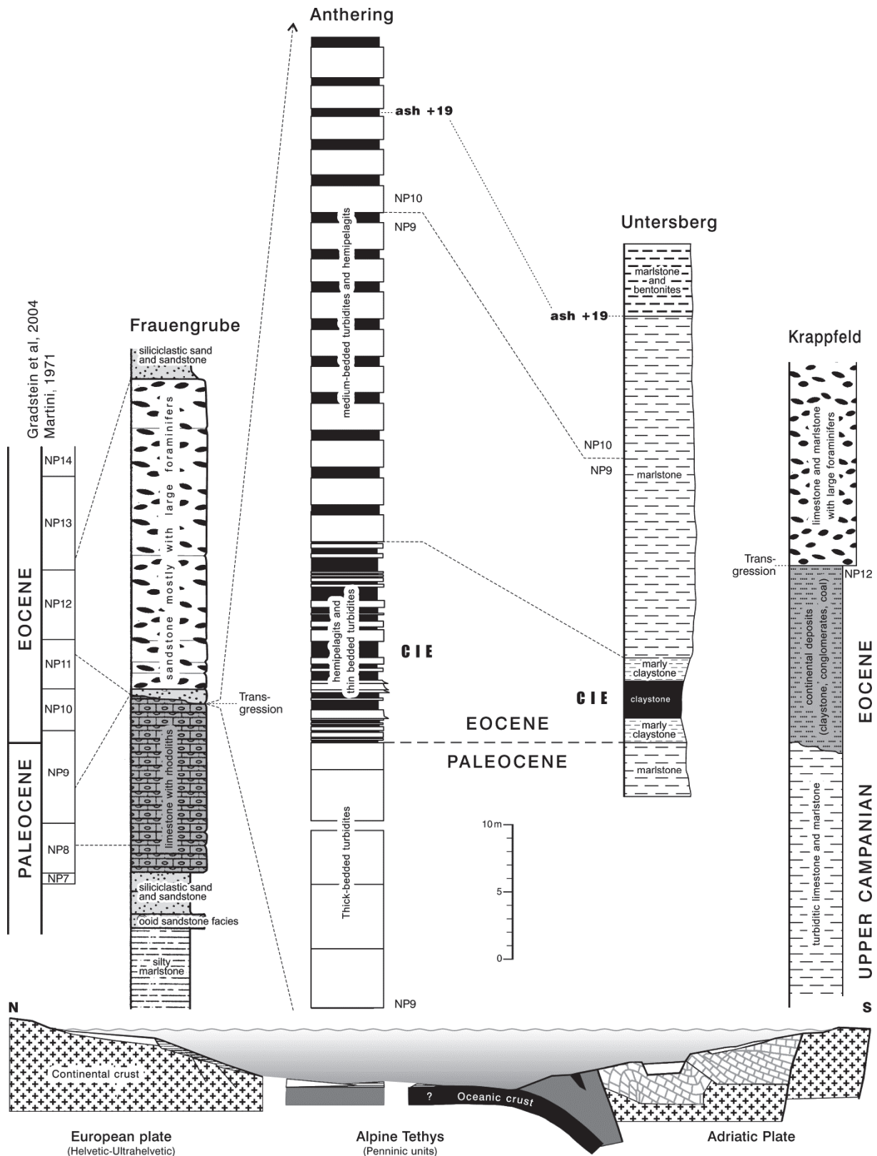
Fig. 2: Correlation and paleogeographic position of Paleogene sections across the Penninic Basin.
