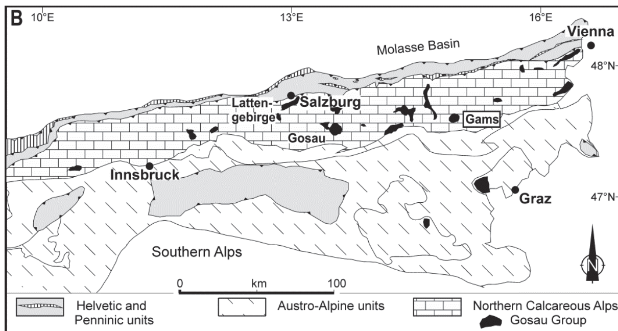
Fig. 5: Location of Gosau deposits in the Eastern Alps.
