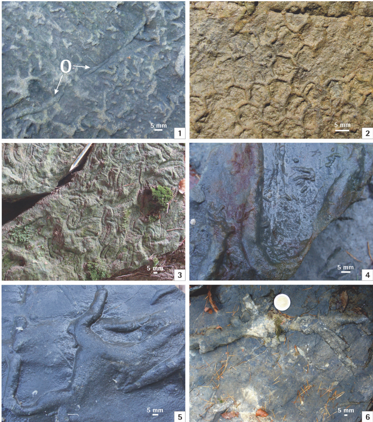
Fig. 28: Ichnofossils from the Thanetian (creek 3) and Ypresian (creek 4) of the Goppling section 1) Ophiomorpha annulata (O) and ? Protopaleodictyon isp. – creek 3; 2) Paleodictyon majus .- creek 4; 3) Scolicia prisca – creek 4; 4) ? Scolicia strozzii – creek 3; 5) Thalassinoides isp. – creek 3; 6) Thalassinoides isp. – creek 3.
