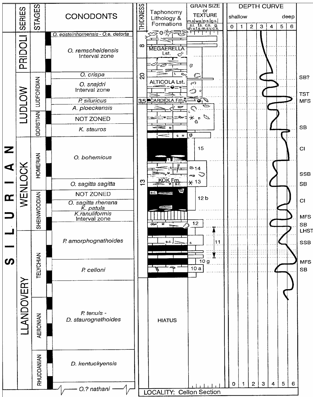
Fig. 35: Conodont stratigraphy, lithology, grain size, significant taphonomic features and depth curve of the Silurian of the Cellaon section. Modified from SCHÖNLAUB, 1997.
