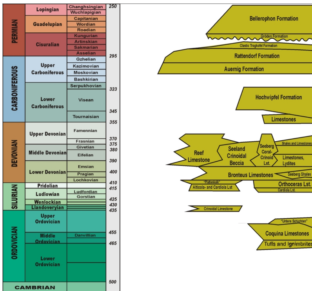
Fig. 11: Biostratigraphic scheme of the Paleozoic sequence of the Karawanken Alps. After SCHÖNLAUB, 1985, modified.
