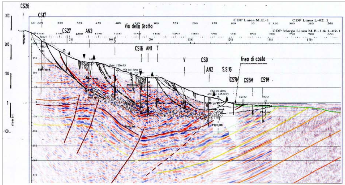
Fig. 3: Geomorphological and seismic section.
