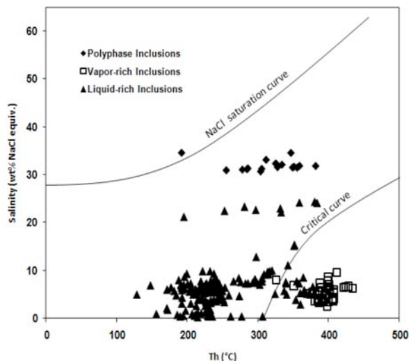
Fig. 2. Distribution of salinity and T_h values for various fluid inclusion types in Baghkhoshk. The NaCl saturation and critical curves from Ahmad and Rose (1980).
