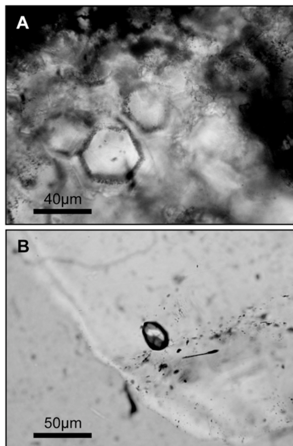
Fig. 2. Fluid and vapour inclusions in sulphosalt-ore stage quartz from the Summitville Au-Ag-Cu deposit, Colorado: (A) primary inclusions (<1 µm) mantling growth bands in euhedral quartz; (B) An isolated low-density vapour inclusion in quartz.
