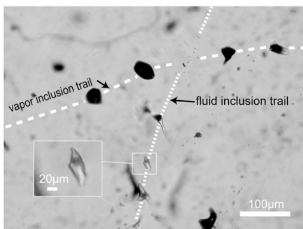
Fig. 1. Crosscutting trails of secondary vapour and secondary fluid inclusions in sulphosalt-ore stage quartz from the Summitville Au-Ag-Cu deposit, Colorado.
