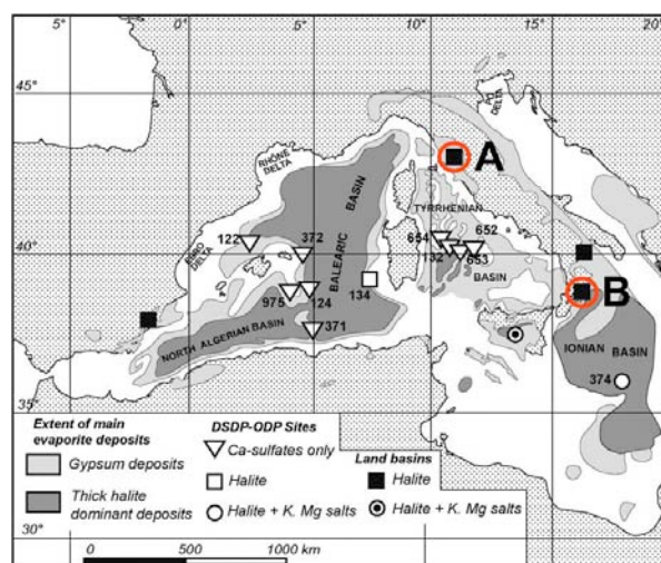
Fig. 1. Map showing distribution and extent of the Messinian evaporites in the Mediterranean area and location of samples (A: Volterra basin; B: Croton basin). Modified from Rouchy & Caruso, 2006.
