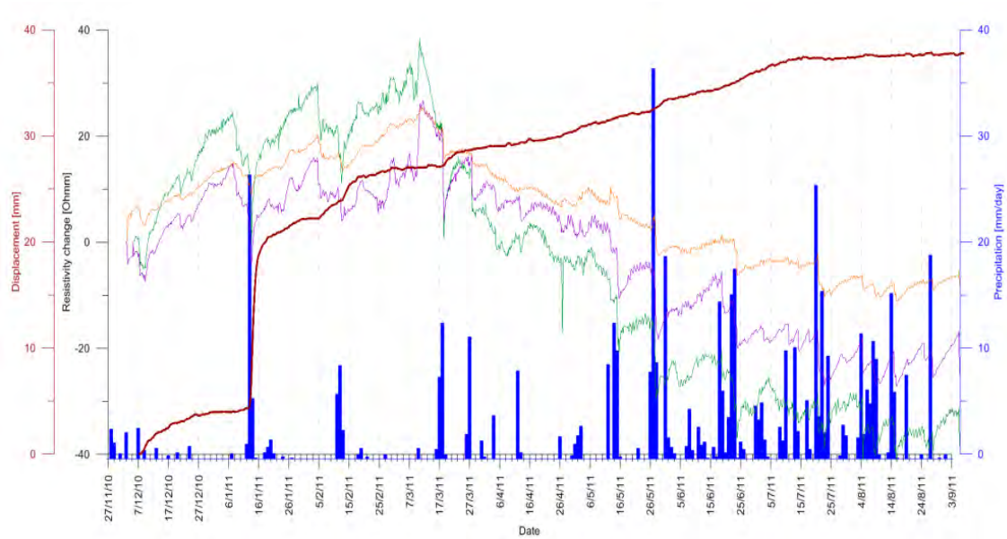
Fig. 6: Display of displacement (red), precipitation (blue; courtesy of the Central Institute for Meteorology and Geodynamics (ZAMG)) and apparent resistivity at different relative apparent depths (green: 1 m; purple: 2 m; orange: 4 m) for the whole survey period.
