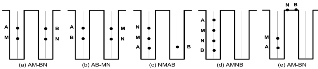
Fig. 8: ERT electrodes arrays: (a-b) Bipole-bipole; (c) Four-electrode gradient array; (d) Wenner – Schlumberger in the same borehole; (e) Surface-to-borehole.
