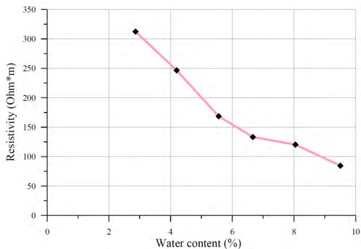
Fig. 6: Resistivity of compacted sand
