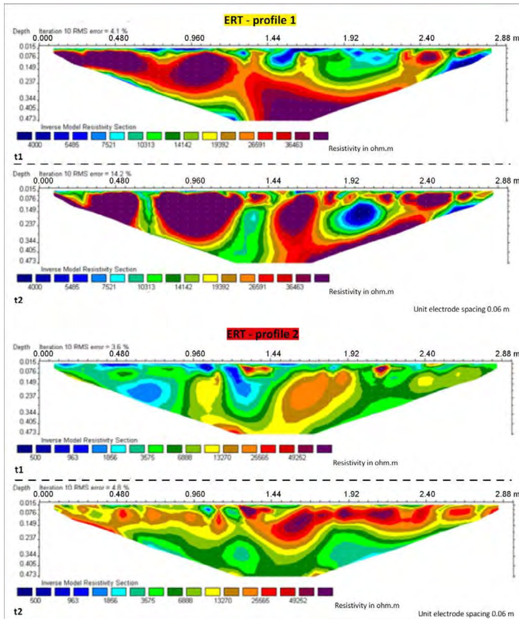
Fig. 4: Inversion models (Wenner-array) of the resistivity values at profile 1 and 2. RMS error: (root-mean-squared-error) = Difference between the calculated and the apparent measured resistivity.
