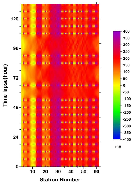
Fig. 1: SP monitoring data were acquired from Feb. 8., 2011, 00:00 to Feb.13., 2011, 12.00 measured every six hours at 62 stations.
