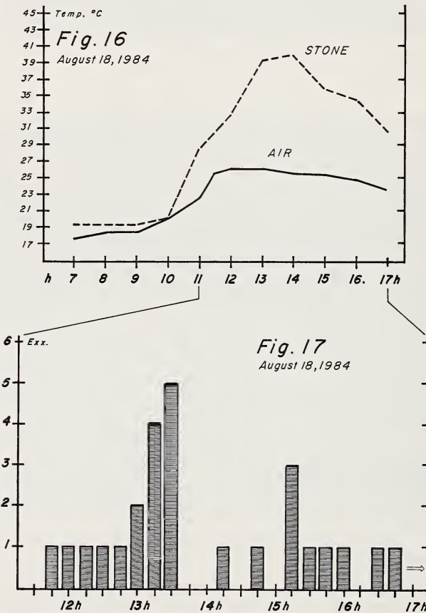
Fig. 16: Thermometric regime of the air and stone surfaces on August 18, 1984 at Gorreta (Hierro).
