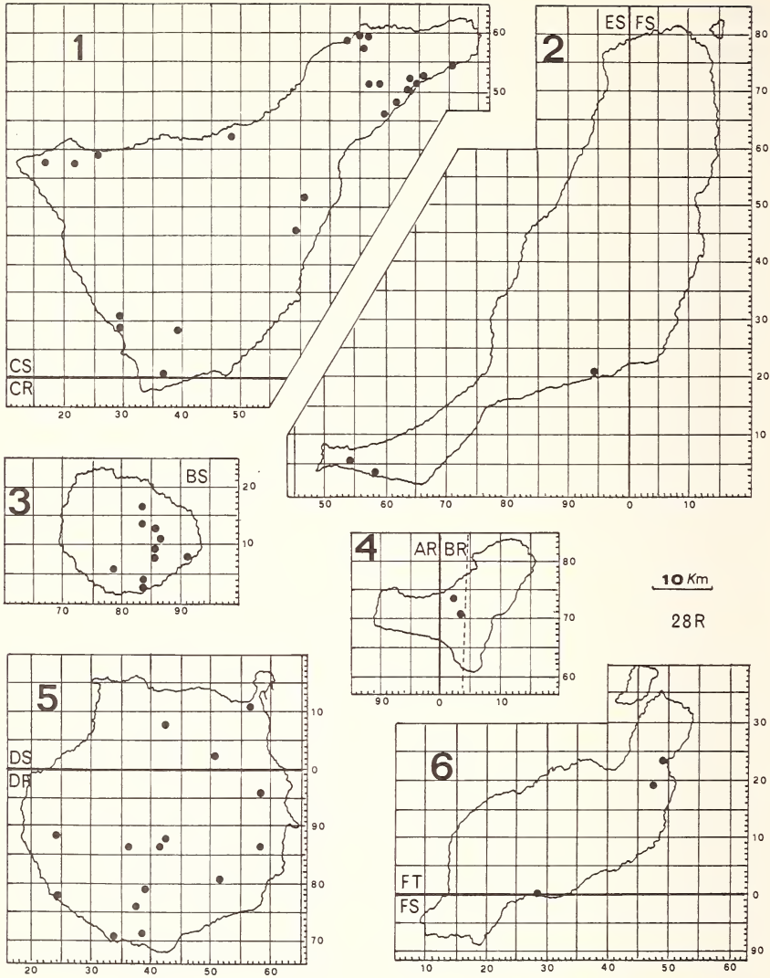
Fig. 2: Distribution of Ocneroдрilus occidentalis in the Canary Islands. Tenerife (1); Gomera (3); Hierro (4); Gran Canaria (5); Fuerteventura (2); Lanzarote (6).
