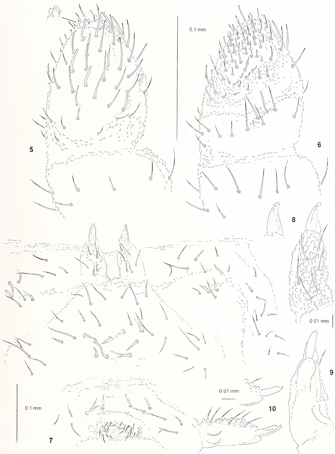
Fig. 5–10. — Pseudachorutella bescidica sp. n. 5. antennal segments II–IV of right antenna, dorsal view. 6. antennal segments II–IV of right antenna, ventral view. 7. furca, genital plate and male ventral organ. 8. furca, dorsal view. 9. furca, ventral view. 10. furca, lateral view.
