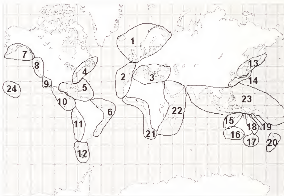
Fig. 1. Map showing biogeographic regions used in the present study. Regions have been modified from BRIGGS (1995). 1. Northeast Atlantic. 2. Lusitanian. 3. Mediterranean (including the Black Sea). 4. Northwest Atlantic. 5. Caribbean. 6. Southwestern Atlantic tropical and warm temperate. 7. Aleutian. 8. Oregonian. 9. Californian. 10. Mexican-Panamanian. 11. Southeastern Pacific warm temperate. 12. Cold temperate South America. 13. Northwest Pacific cold temperate. 14. Northwest Pacific warm temperate. 15. Northern and northwestern Australia. 16. Southwestern and southern Australia. 17. Southeastern Australia. 18. Northeastern Australia. 19. Great Barrier Reef. 20. New Zealand. 21. Southeast Atlantic. 22. Western Indian Ocean. 23. Indo-Polynesian region (including Ryukyu Islands). 24. Hawaii.
