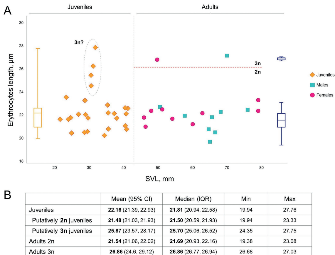
Fig. 1. A. The distribution of frogs from the Zone by their mean erythrocyte lengths vs body length (SVL). Red dash line marks putative cut-off value for adult triploids; dash circle marks juveniles of doubtful ploidy. Boxplots denote means (middle line), IQRs (boxes) and extreme values (whiskers). B. The sample parameters for different groups of studied frogs.
